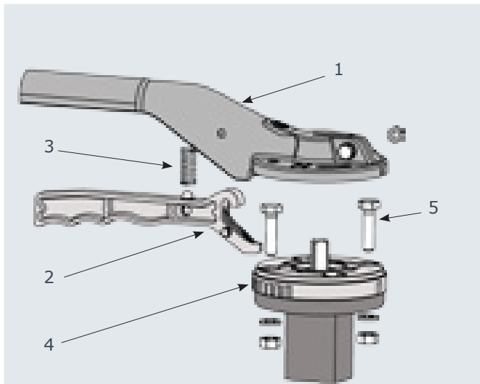
Adjustable handlever
