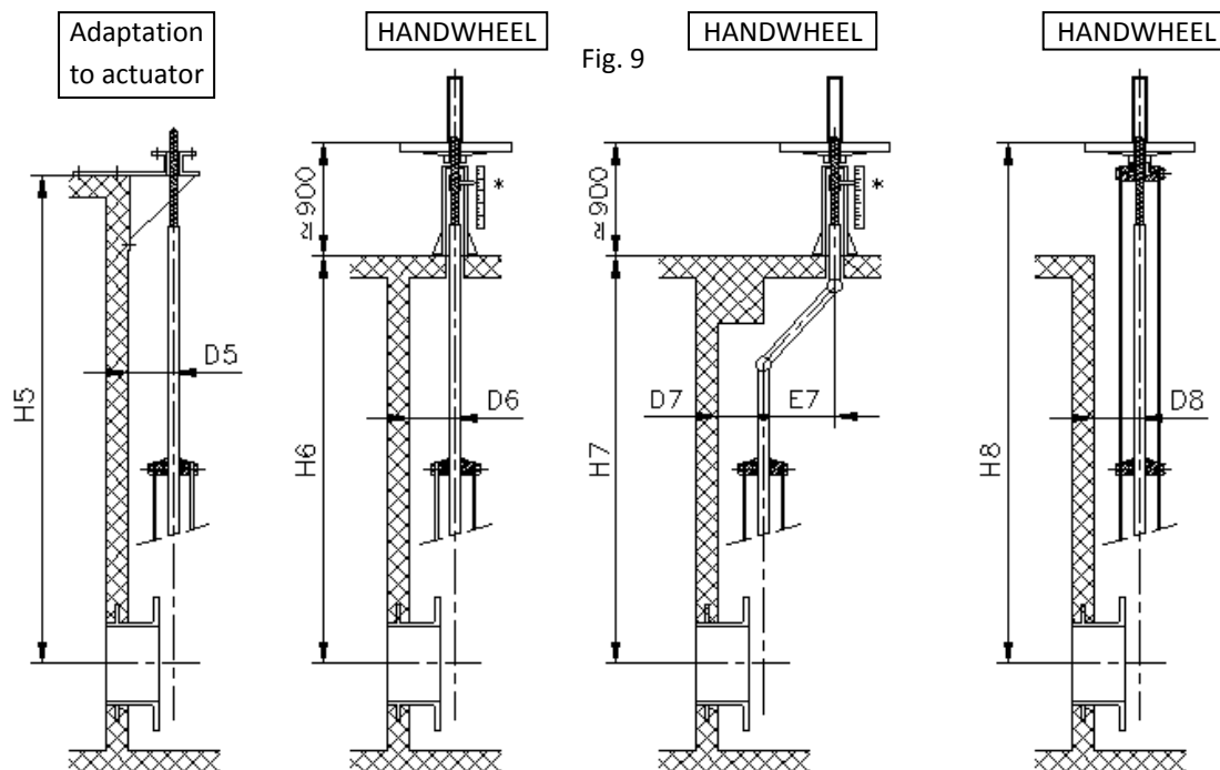
5- Rising stem + bracket support + adaptation to actuator.
