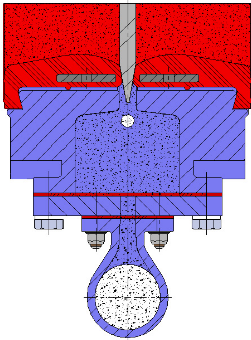
SECTION E-E
