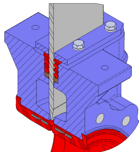
DETAIL C
